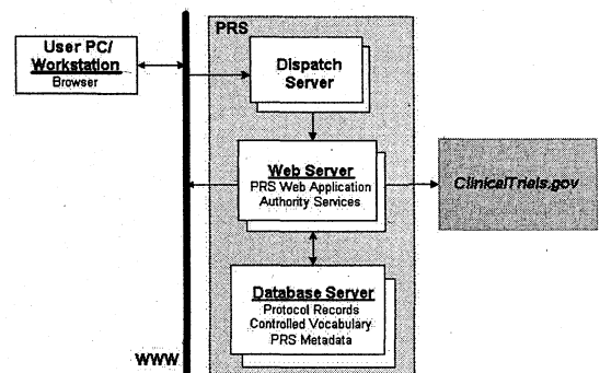
Figure 2 - Protocol Registration System Architecture
