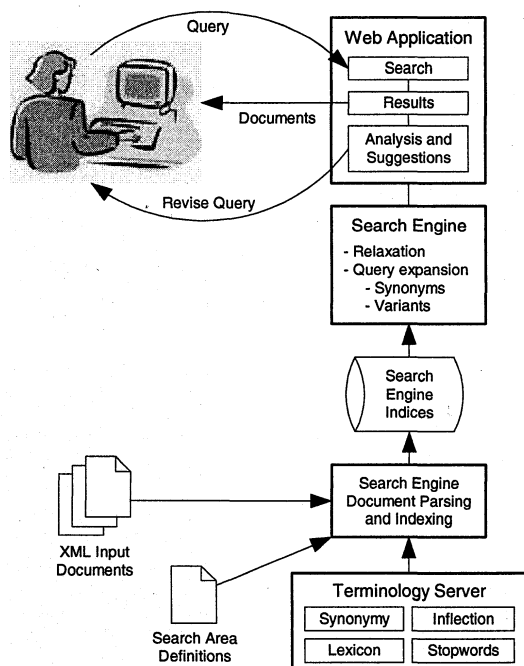
Figure 1 - SE search and retrieval system
