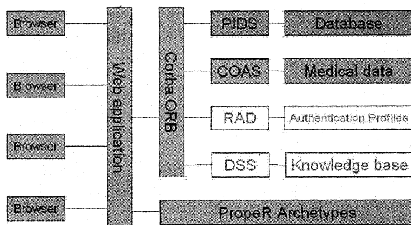
Figure 1 - Proper EHR diagram.
