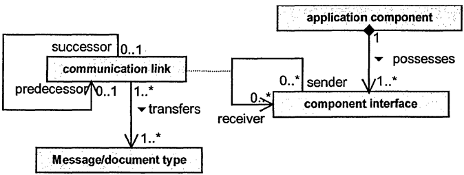
Figure 3: A UML-based meta model for a 3LGM 2 communication process.
