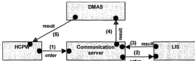
Figure 4: An example of a communication process (HCPW: healthcare professional workstation; LIS: laboratory information system; DMAS: documents management and archiving system). Black circles represent communication interfaces; arrows represent communication links; numbers in round brackets represent the sequence of communication links, the labels of the arrows represent the message types transmitted.
