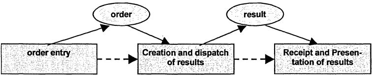
Figure 2: Example of a 3LGM 2 business process. (Ovals: entity types; rectangles: enterprise functions). The enterprise functions are taken from [10].
