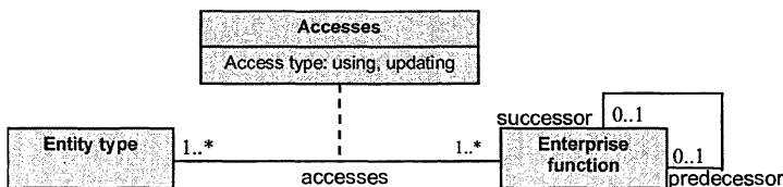
Figure 1: A UML-based meta model for 3LGM 2 business processes.
