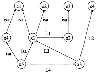
Figure 1: Find relation via path algorithm
