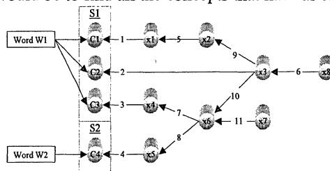
Figure 2 : Starting search from terms
