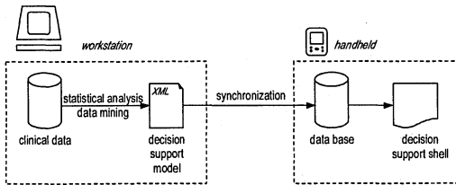
Figure 1 Handheld-based decision support system
