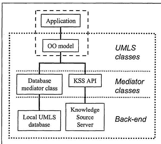
Figure 3 - Architecture of the model
