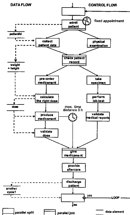
Fig. 1: Modeling of Processes in ADEPT
