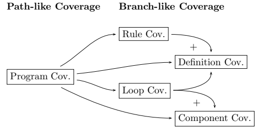
Figure 1. Relations between total coverage of different notions.
