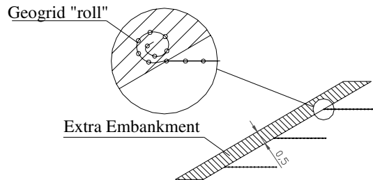
Figure 3. Geogrid installation and placement of extra embankment.
