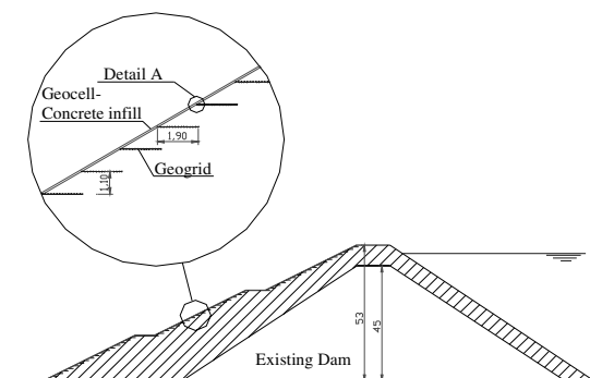
Figure 2. Cross section of the Dam.
