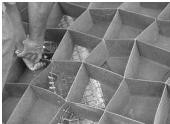
Figure 8. Stapling process.
