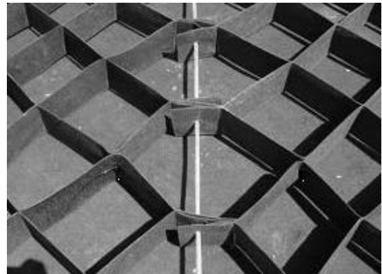
Figure 5. Transversal joints.
