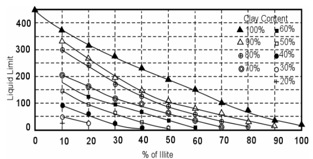
Figure 3. Variation of liquid limit of the mixture of quartz, illite, and montmorillonite with the proportion of illite
