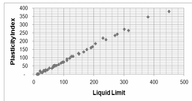
Figure 1. Relationship between plasticity index and liquid limit of the tested mineral mixtures
