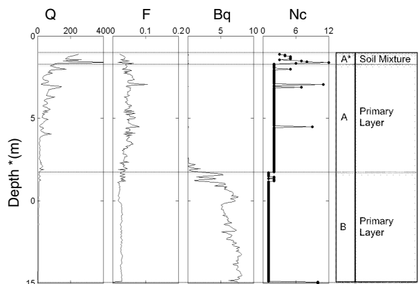
Figure 3. CPTu sounding C-079 through dyke crest, normalized tip resistance (Q, F, Bq) and stratigraphic delineation from three-dimensional cluster analysis.
