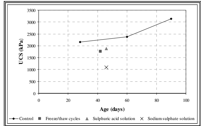
Figure 3. UCS results of the stabilised clay mix 1 in the aggressive and control environments
