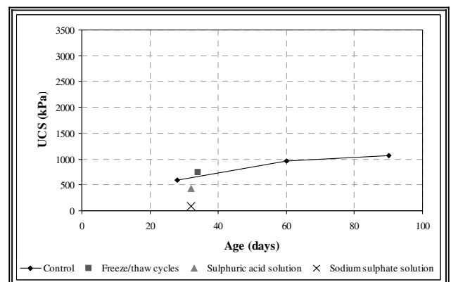
Figure 4. UCS results of the stabilised clay mix 5 in the aggressive and control environments
