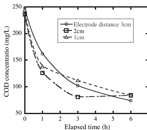
Figure 4. Relationship between COD concentration and elapsed time.
