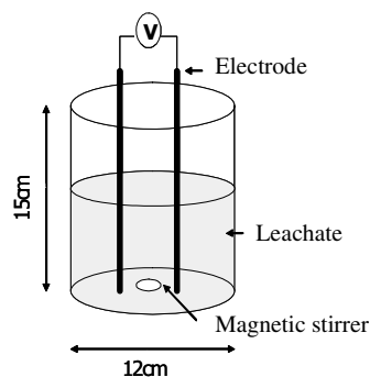
Figure 3. Schematic diagram of the electrolytic apparatus.
