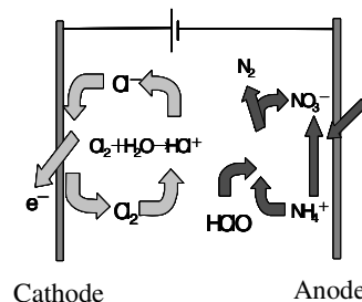
Figure 1. Fundamental principle of the oxidation processes.
