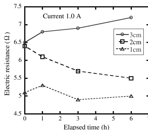
Figure 5. Relationship between electric resistance and elapsed time.
