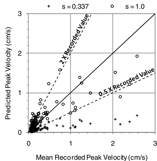
Figure 5. Predicted versus recorded peak velocity.
