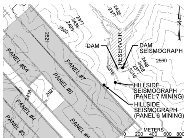
Figure 1. Basic site layout.
