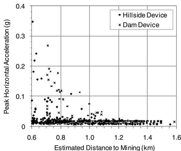
Figure 3. Peak acceleration versus estimated distance to mining.
