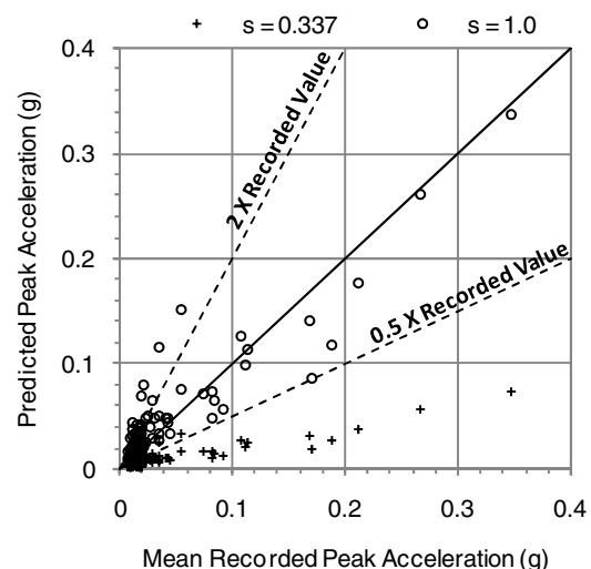
Figure 6. Predicted versus recorded peak acceleration.
