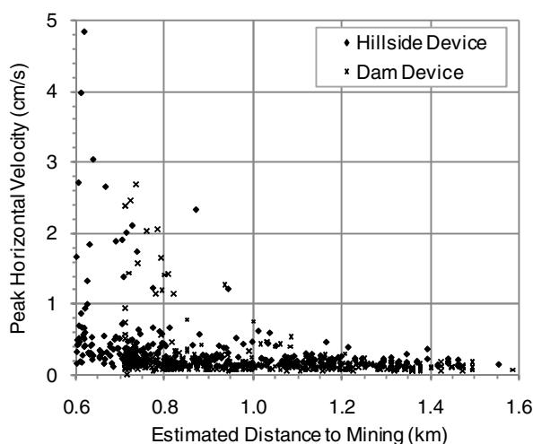
Figure 2. Peak velocity versus estimated distance to mining.
