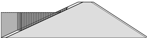
Figure 5. A typical slip surface in the upstream slope of the dam.
