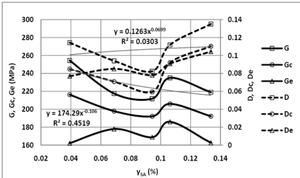
Figure 6. Variation of shear modulus and damping ratio with shear strain for sample with M.A.S. = 25.4 mm, b=6% and \sigma_3=600 kPa
