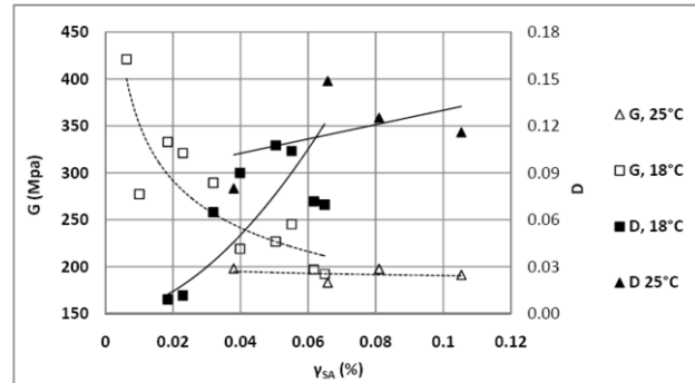
Figure 9. Effects of temperature on G and D, M.A.S.=12.7 mm, b =5.5% and \sigma_3=400 kPa
