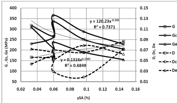
Figure 5. Variation of shear modulus and damping ratio with shear strain for sample with M.A.S. = 25.4 mm, b=5% and \sigma_3=600 kPa
