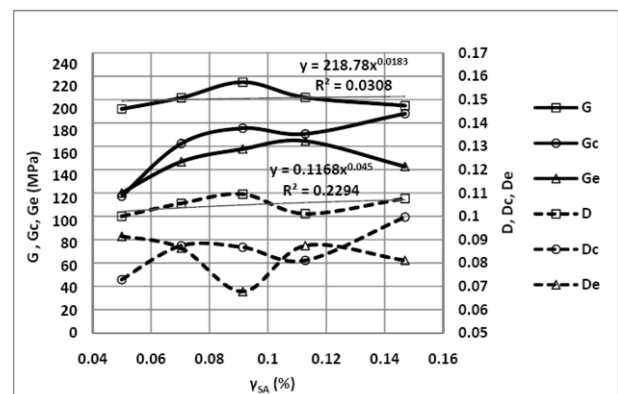
Figure 4. Variation of shear modulus and damping ratio with shear strain for sample with M.A.S. = 12.7 mm, b=5.5% and \sigma_3=600 kPa
