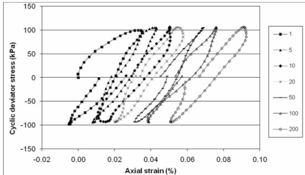
Figure1. Hysteresis loops for test on sample with M.A.S.=25.4 mm, b=5%, \sigma_3=200 kPa, \sigma_d=200 kPa, T=25^\circ\text{C}
