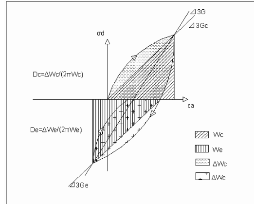
Figure 3. Calculation of G_c , D_c , G_e , D_e
