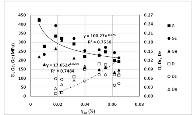
Figure 8. Variation of shear modulus and damping ratio with shear strain, M.A.S.= 12.7 mm, b= 5.5%, \sigma_3=400 kPa and T= 18°C
