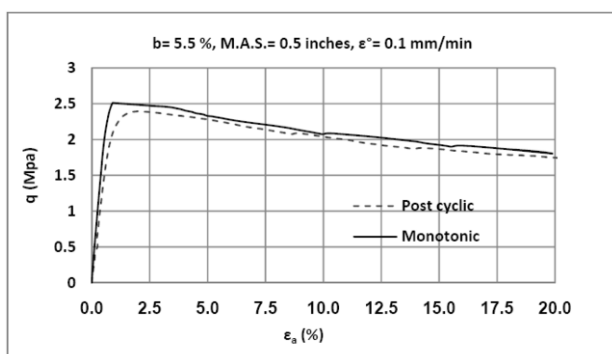
Figure 11. Stress- strain curves obtained from monotonic and post-cyclic tests on sample with M.A.S.= 12.7 mm and b= 5.5%
