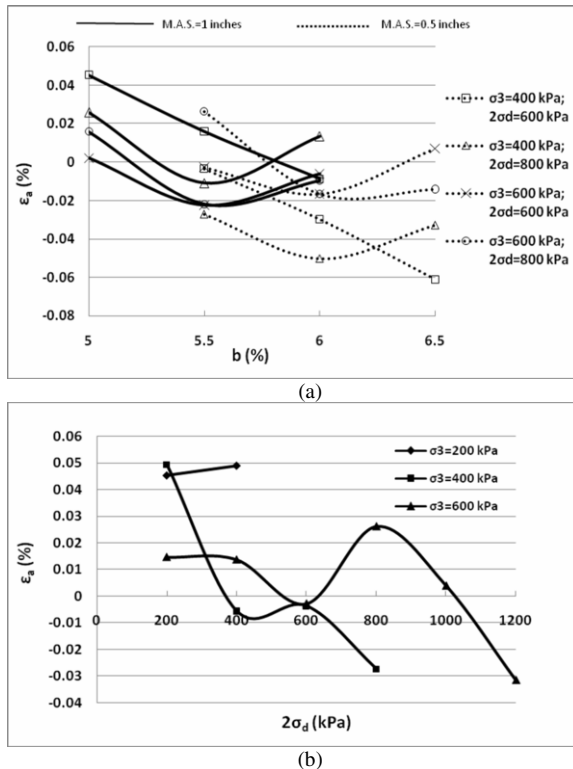
Figure2. Variation of remained strain after 199 cyclic loading with a) bitumen content; b) deviator stress and confining pressure for M.A.S.=12.7 mm and b=5.5% at T=25^\circ\text{C}
