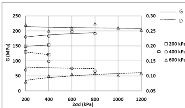
Figure 7. Effects of confining pressure and deviator stress on G and D, M.A.S. = 25.4 mm, b= 5.5 % and T= 25°C
