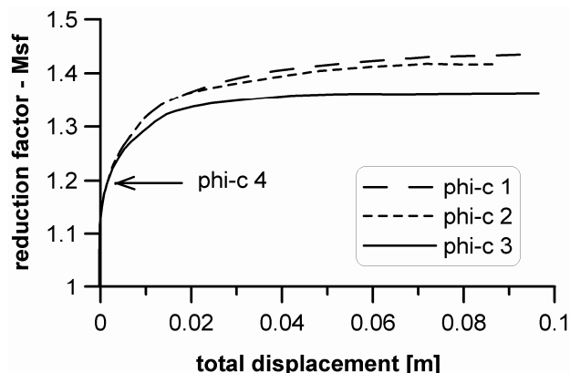
Figure 5 Development of the \phi -c reduction factor with wall displacements after the last construction stage using different assumptions on the strength of structural elements: infinite strength (1), ductile strength of the wall only (2), ductile strength of the wall and anchor tendons (3), ductile strength of the wall and brittle strength of anchor tendons (4).
