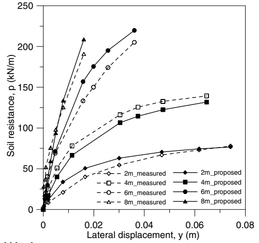
(a) Field load test
