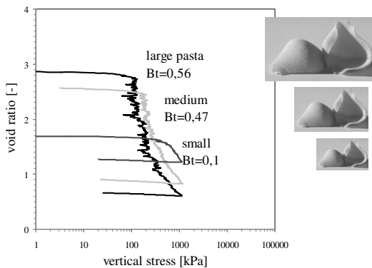
Figure 3. Impact of the grain size on the breakage
