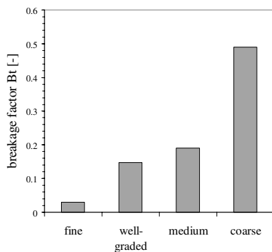
Figure 7. Breakage factor of fine, medium and coarse uniformly-graded and well-graded carbonate sands
