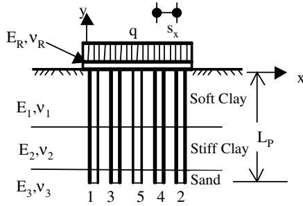
Figure 2. Geotechnical model for case study 2.
