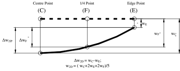
Figure 4. Definition of raft settlement for the 2-D Case
