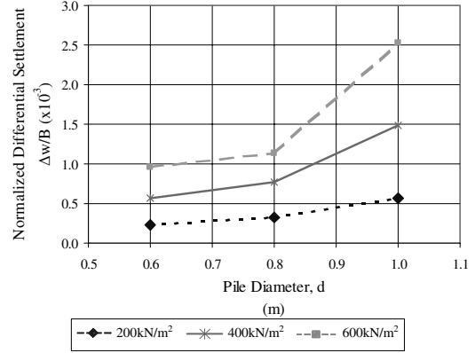
Figure 7. Normalized differential settlement vs. pile diameter
