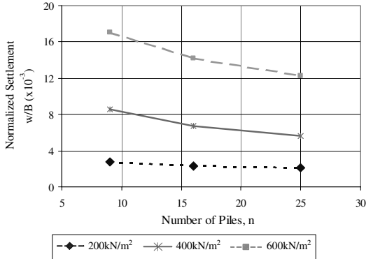
Figure 6. Normalized settlement vs. no. of piles.
