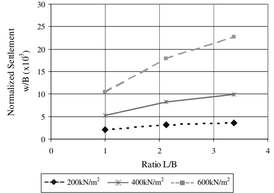
Figure 8. Normalized settlement vs. raft dimension ratio (Case 4)
