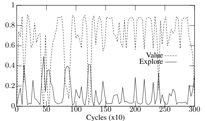
Figure 2. Activities of the Value and Explore modules in one experiment.
