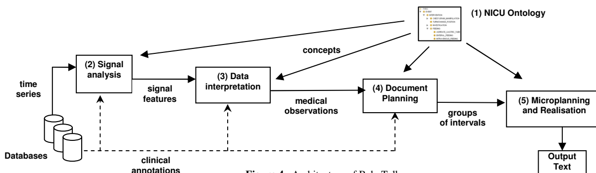
Figure 4. Architecture of BabyTalk
