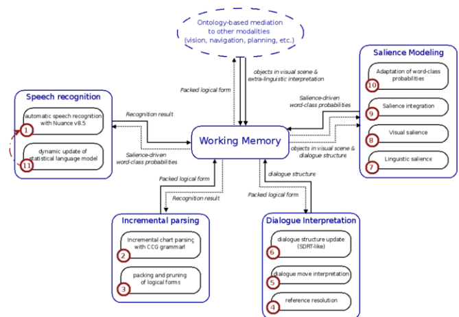
Figure 3. Schema of the system for spoken dialogue comprehension
