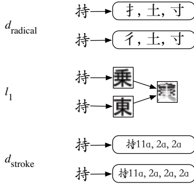
Figure 1. A visual overview of the three distance metrics. For d_{\text{radical}} , a token representing each radical present is used. For l_1 , the images are rendered and the sum of the difference image is calculated. For d_{\text{stroke}} , the edit distance between stroke code vectors is used.
