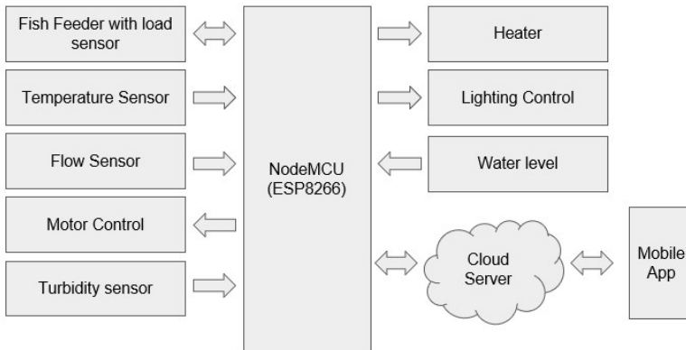
Figure 1. Block Diagram
